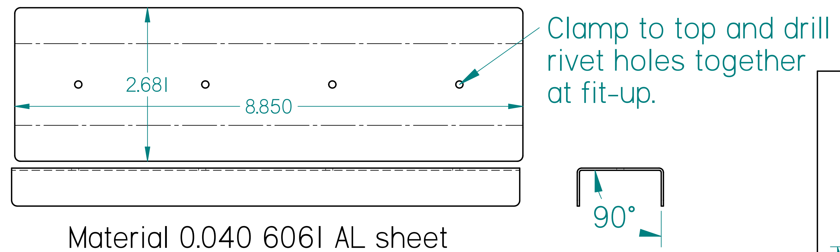
Flat pattern for top reinforcing channel
