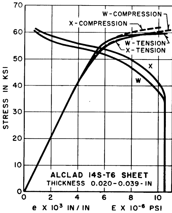
Figure 3.113 (b). Typical stress-strain and tangent compression modulus curves for 14S aluminum alloy sheet.
