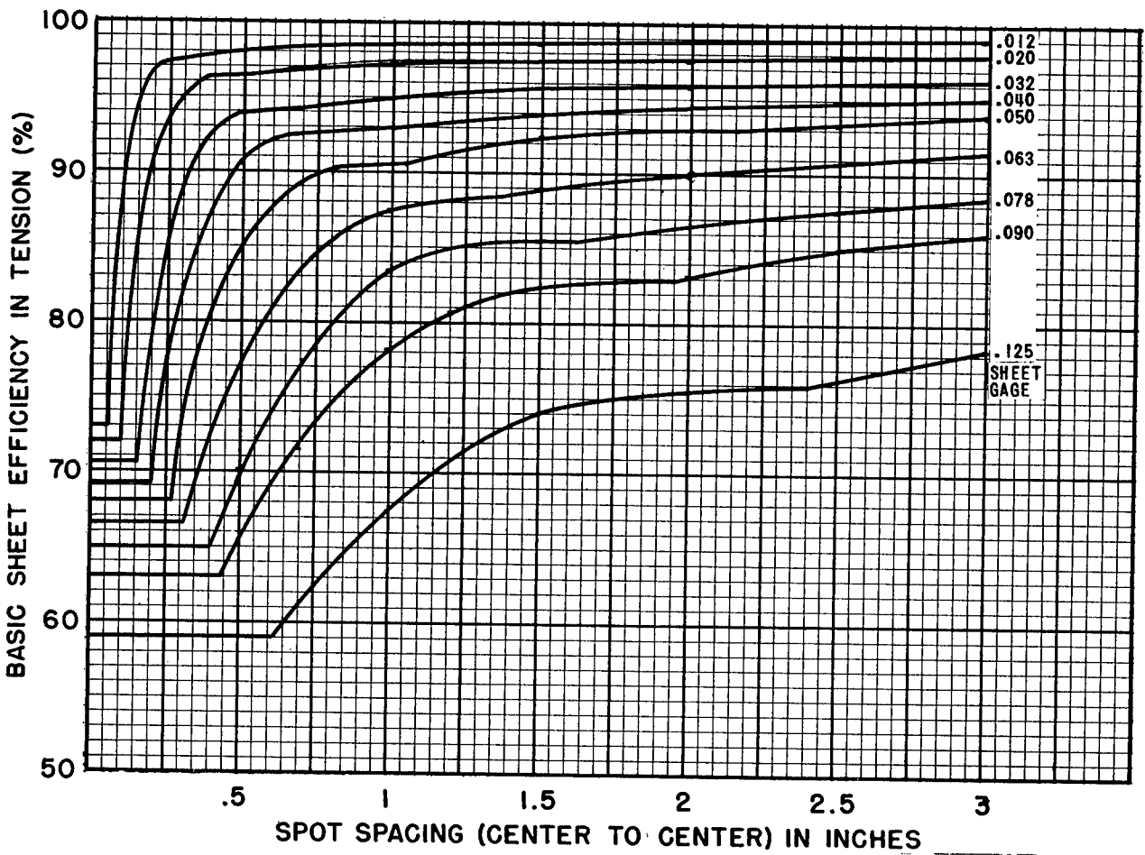
40 Figure 2.61261 (c). Efficiency of the parent metal in tension for spotwelded 302-H corrosion resisting steel.
