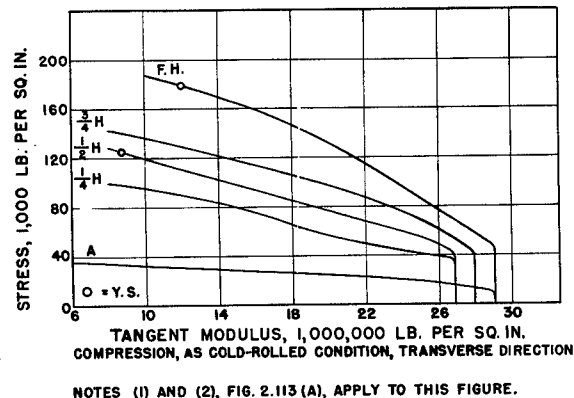
FIGURE No. 2.113 (b)
