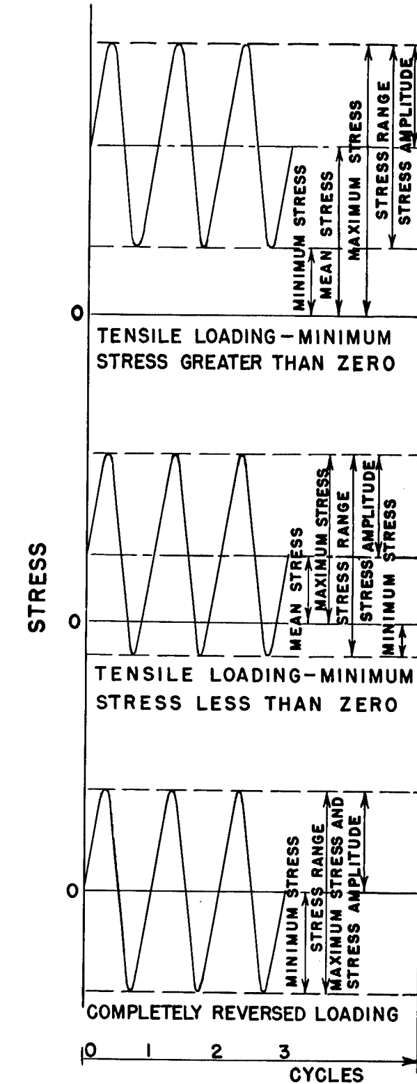
Figure 1.481. Typical fatigue loadings.
