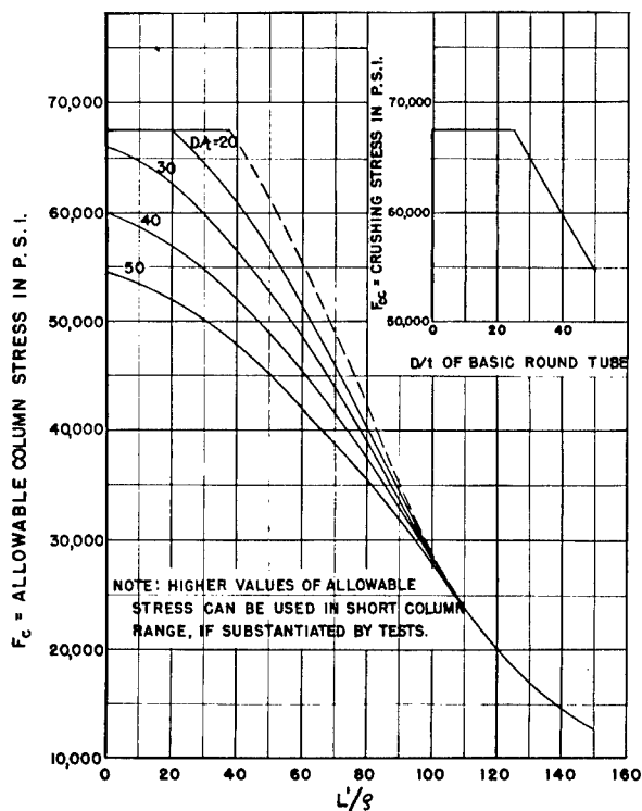
Figure 2.23 (b). Allowable column and crushing stresses for chrome molybdenum streamline tubing F_{1y} = 75,000 p. s. i.
