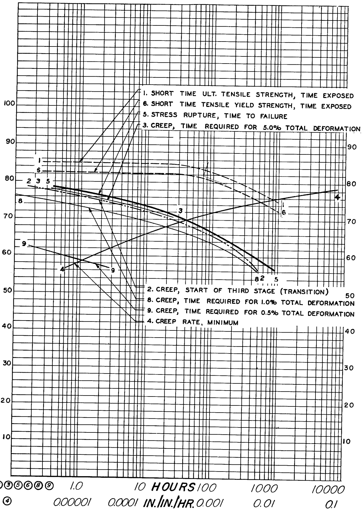
Figure 3.1221 (l). Elevated temperature properties of clad 24S-T86 aluminum alloy (heat treated, cold worked, and aged) at 300° F.
