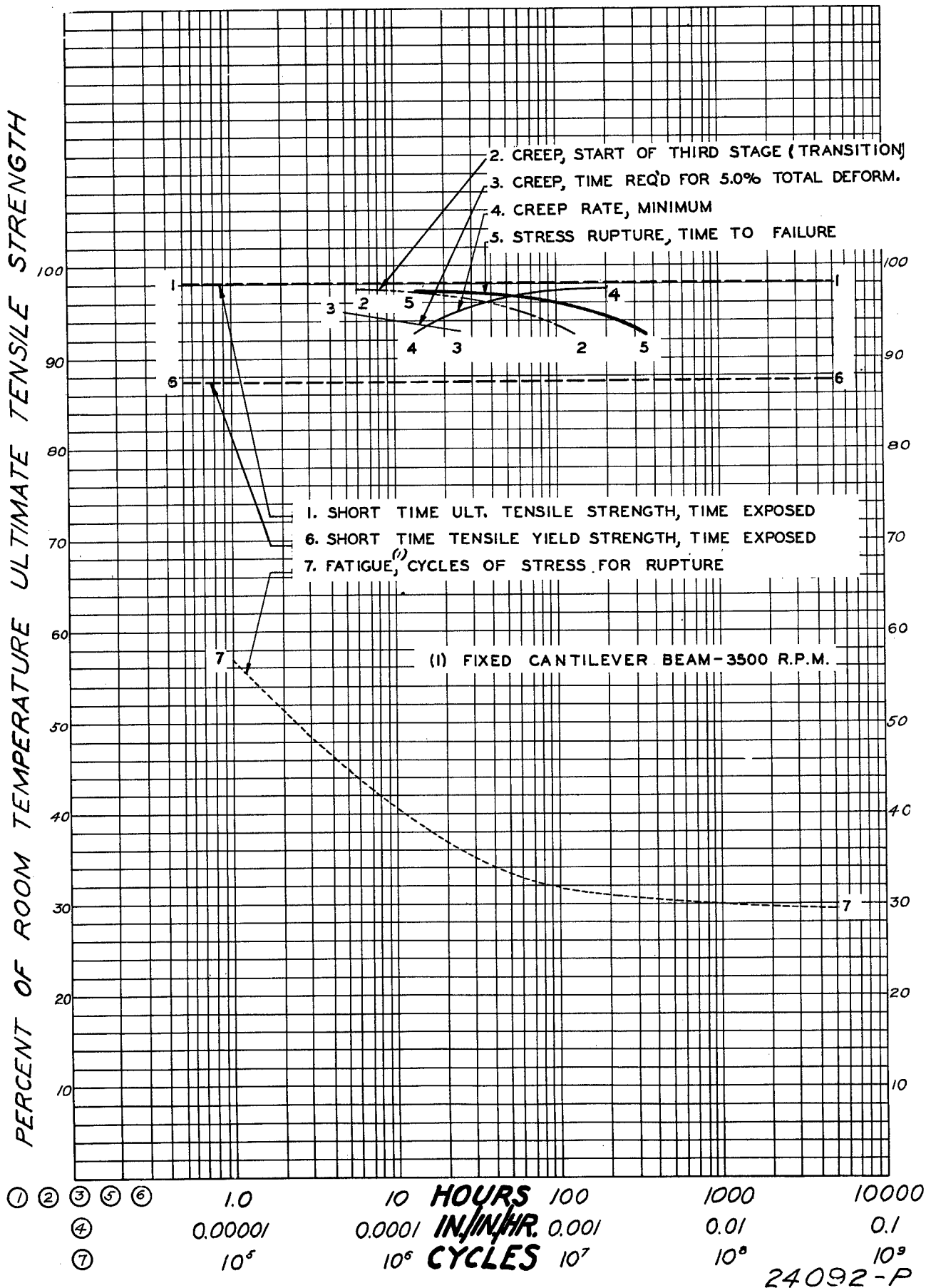
Figure 3.1221 (g). Elevated temperature properties of wrought 75S-T6 aluminum alloy at 94° F. 71
