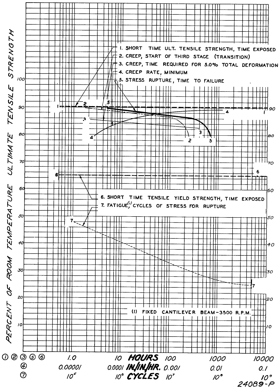
Figure 8.1221 (d). Elevated temperature properties of wrought 24S-T3 aluminum alloy at 211° F.
